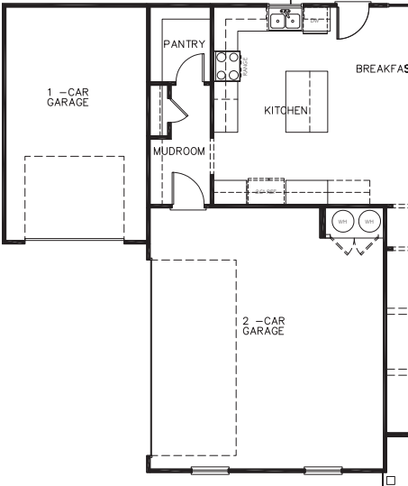
OPTIONAL 3 RD CAR BOLT SIDE ENTRY
