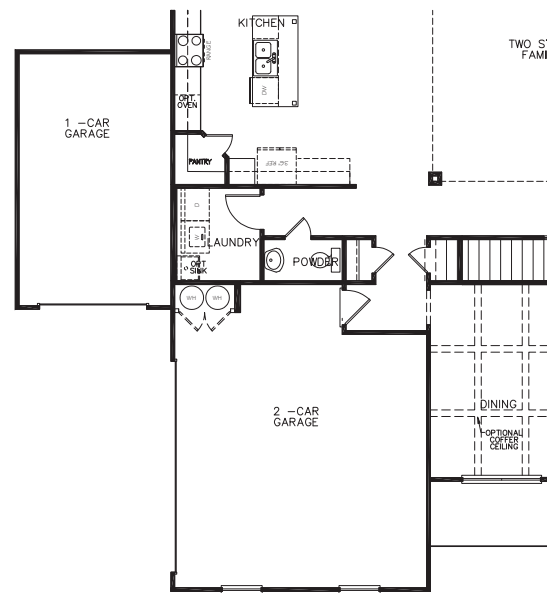
OPTIONAL 3 RD CAR BOLT SIDE ENTRY
